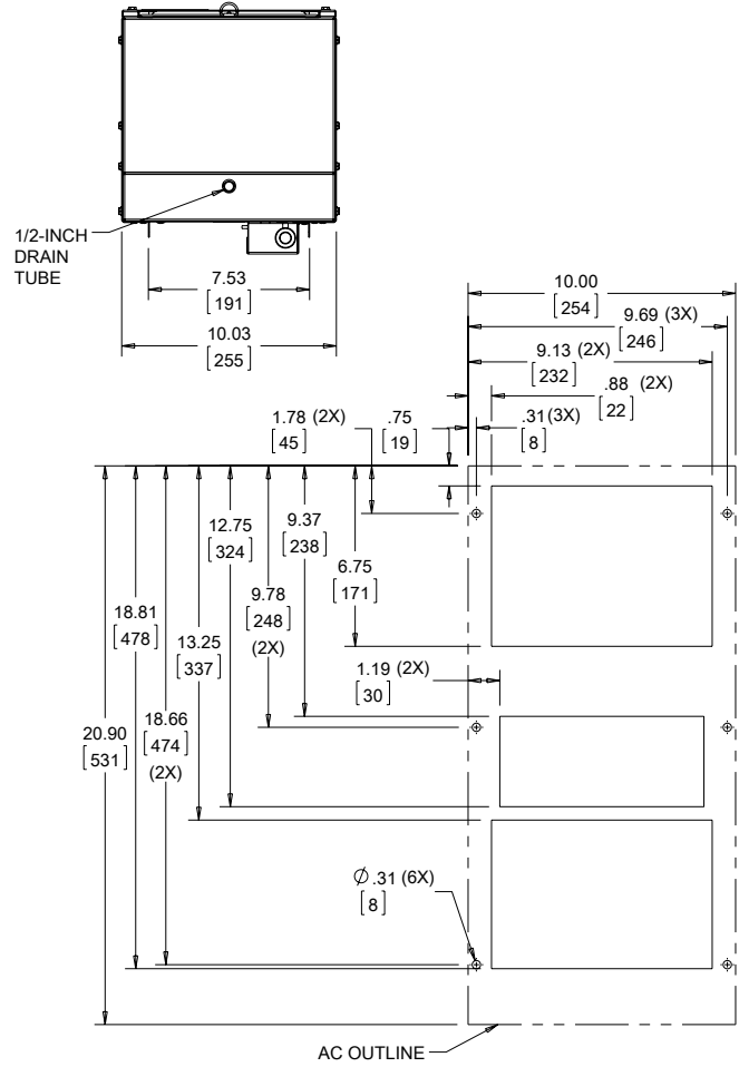
Cutout Dimensions (Externally Mounted)
