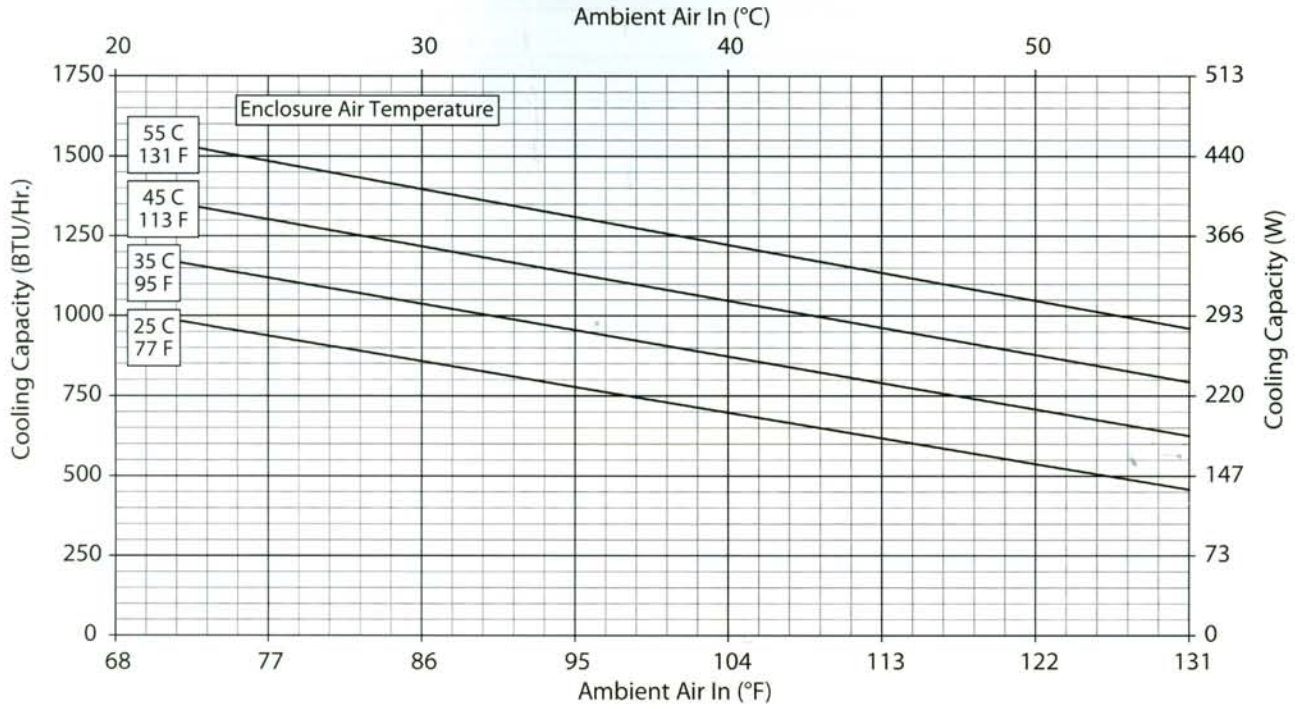
T15-01x6-Gxxx Capacity Curves 60 Hz
