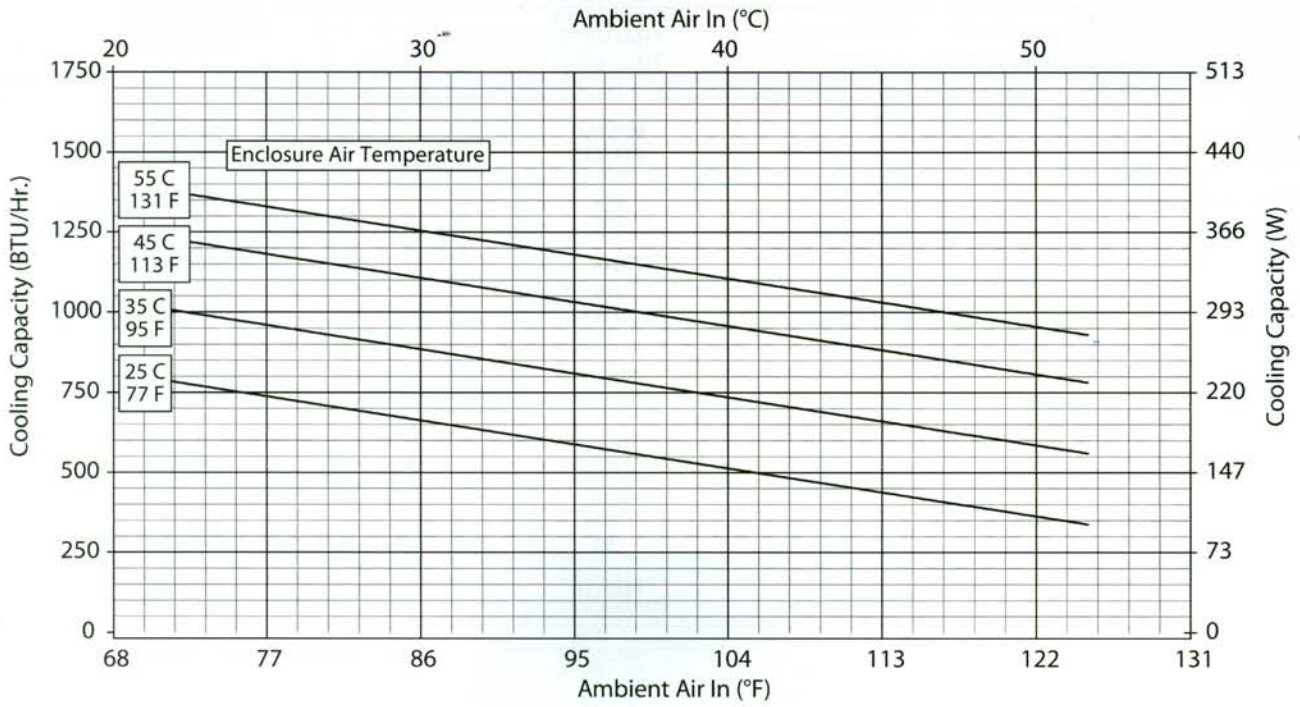
T15-01x6-Gxxx Capacity Curves 50 Hz
