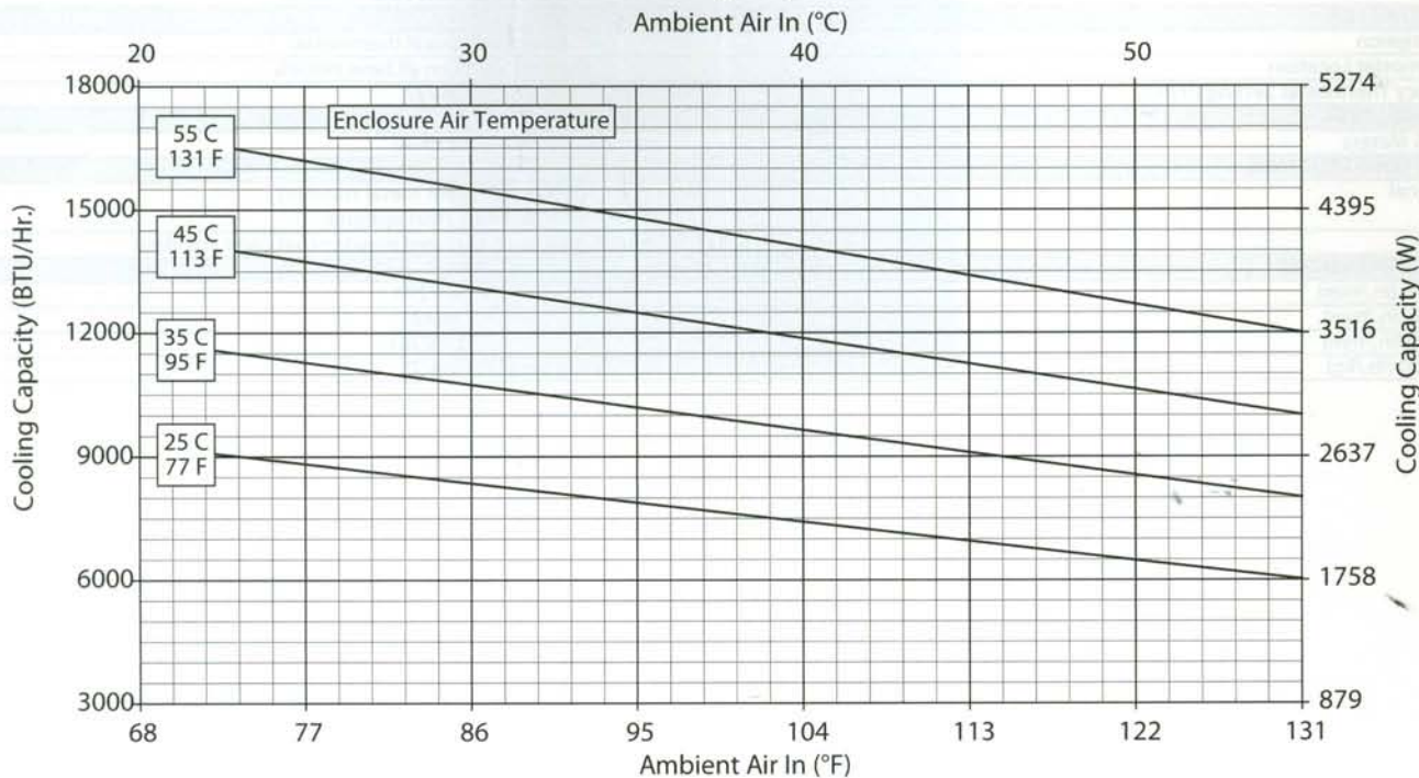
T50-12x6-GXXX Capacity Curves 60 Hz
