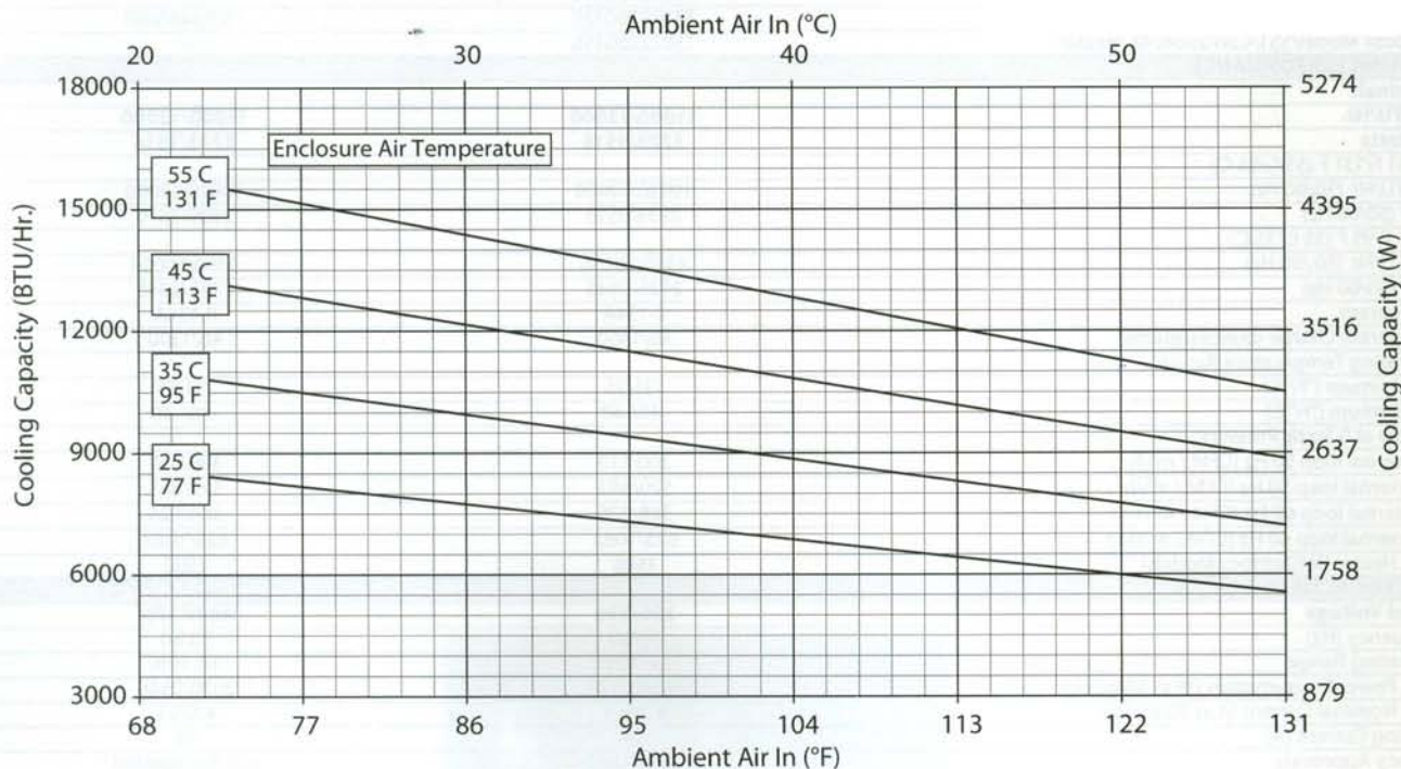
T50-12x6-GXXX Capacity Curves 50 Hz
