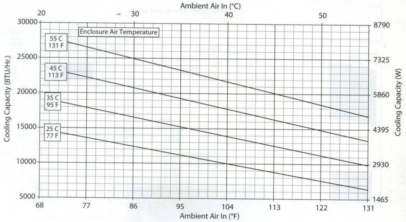
T53-19x6-GXXX Capacity Curve 50 Hz
