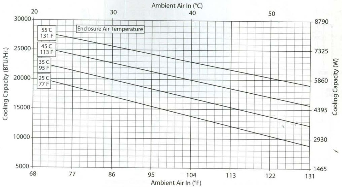
T53-19x6-GXXX Capacity Curve 60 Hz
